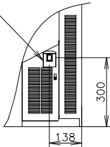
VIEW A(1/10)
